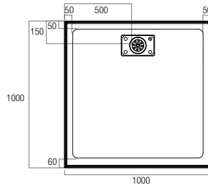
MT1000R
