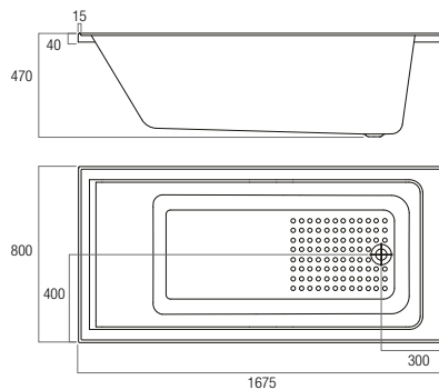
UB1675 1675x800x470
