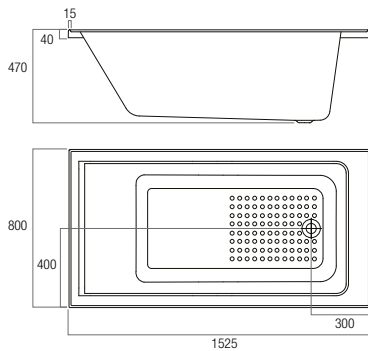
UB1500 1525x800x470
